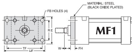
1.50" - 6.00" bores
