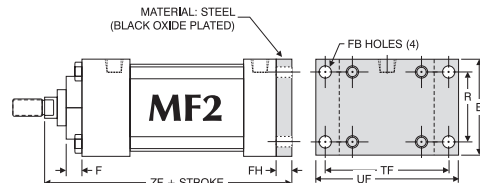
1.50" - 6.00" bores
