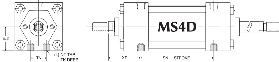
MS4 Bottom Tapped Mount Dimensions
