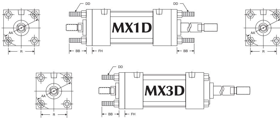
Tie Rod Extended MX1D & MX3D Mount Dimensions
